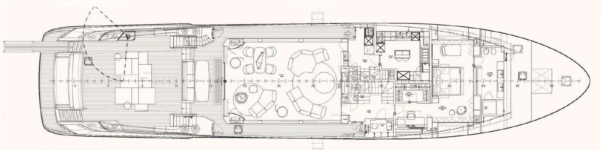
MAIN DECK
