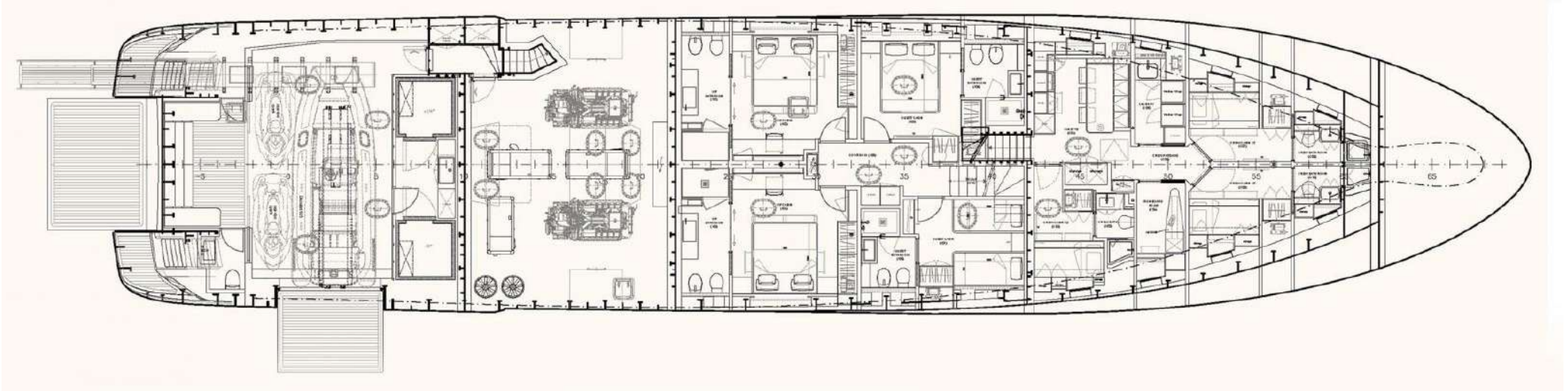
LOWER DECK
